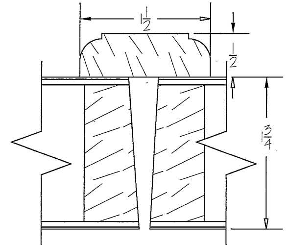
Flat Astragal
