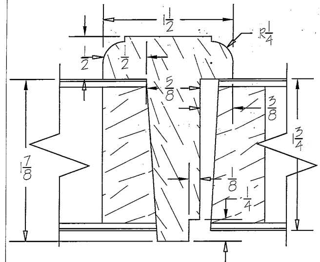
Flat Astragal
