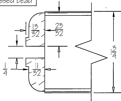
103 recessed bead
